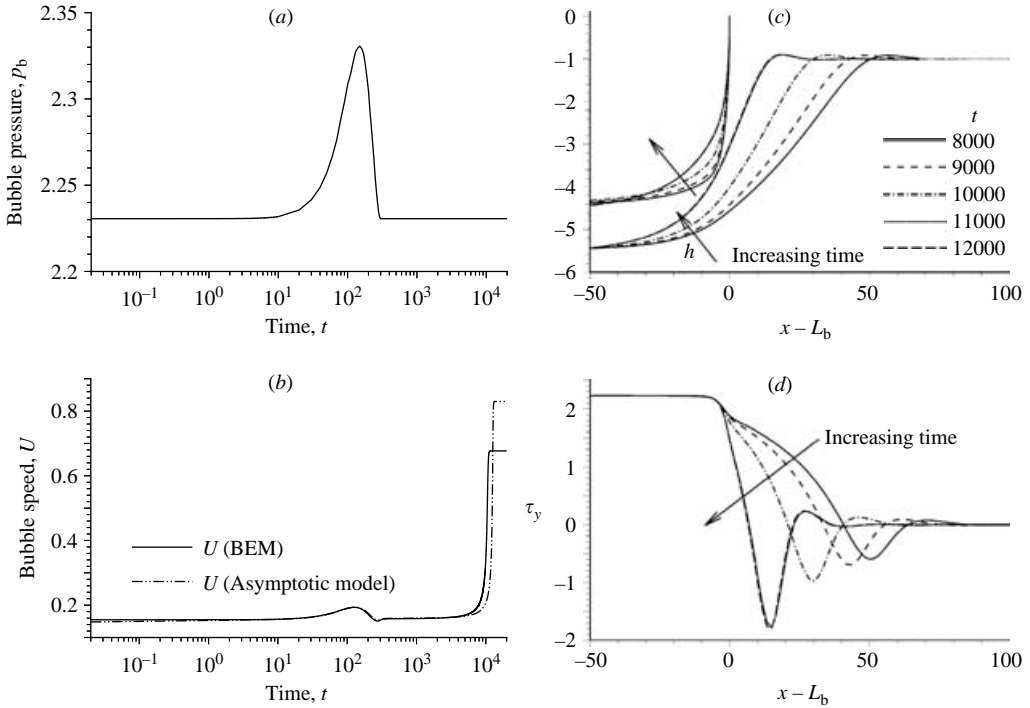
FIGURE 6. The effect of a positive pressure perturbation ( \Delta p = 0.1 , \Delta t = 300 ) on the steady pushing solution with p_{b0} = 2.23 , showing evolution towards steady peeling; other parameter values as for figure 5. (a) p_b and (b) U versus t ; (c) membrane and bubble shapes and (d) vertical stress versus x - L_b , at t = 8000, 9000, 10000, 11000 and 12000 , obtained using BEM calculations.
